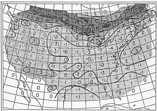
Fig. 2. Storminess at sunspot maxima vs. minima.
